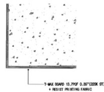
4 CORNER SECTION DETAIL SCALE 1/10
