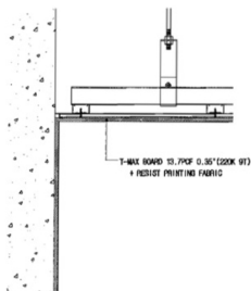
2 WALL-CEILING JOINT SECTION DETAIL SCALE 1/10
