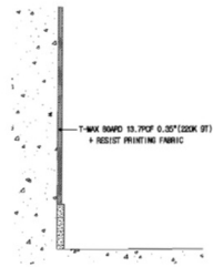
5 BOTTOM SECTION DETAIL SCALE 1/10
