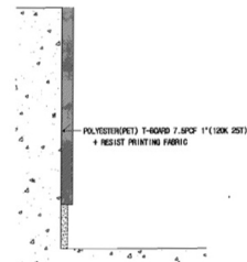
5 BOTTOM SECTION DETAIL SCALE 1/10
