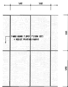
1 T-MAX T-BOARD CEILING & WALL PLAN SCALE None
