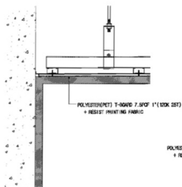
2 WALL-CEILING JOINT SECTION DETAIL SCALE 1/10
