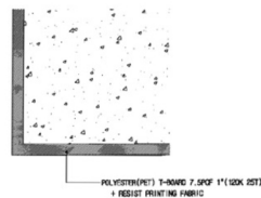
4 CORNER SECTION DETAIL SCALE 1/10
