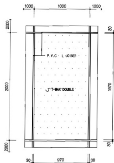
1 T-MAX CEILING & WALL PLAN SCALE None
