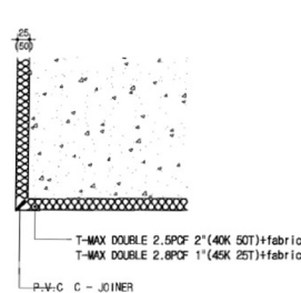
4 CORNER SECTION DETAIL SCALE 1/10
