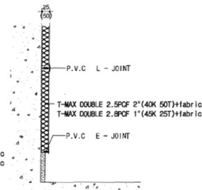
5 BOTTOM SECTION DETAIL SCALE 1/10
