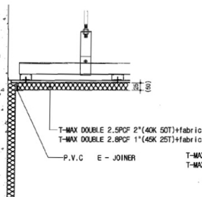
2 WALL-CEILING JOINT SECTION DETAIL SCALE 1/10
